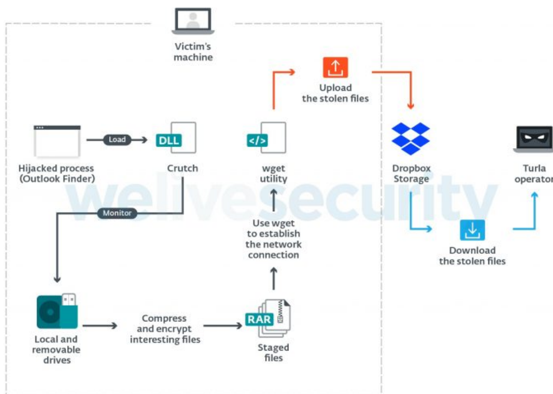
Figure 4. Architecture of Crutch v4
